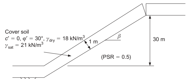
Figure 14. Diagram of the model used in the veneer stability analysis
