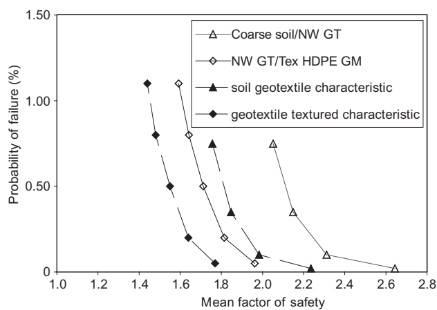
Figure 18. Probability of failure against factor of safety for waste body stability, showing the relationship between the mean and characteristic values for factor of safety, based on combined data
