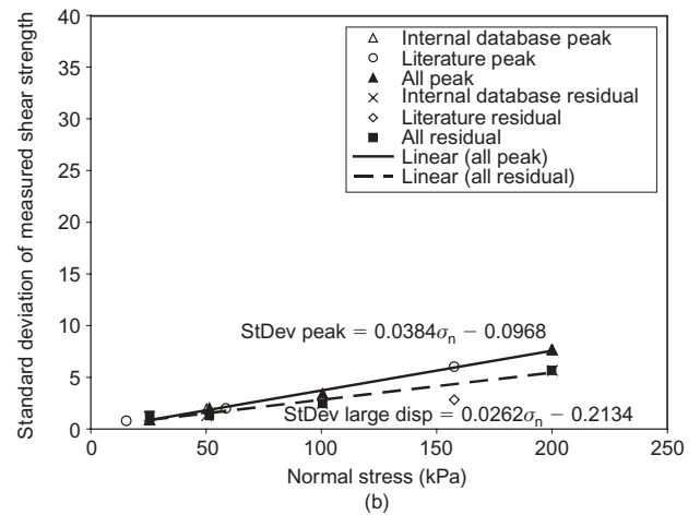
Figure 9. Smooth HDPE geomembrane/nonwoven geotextile from internal database, literature, and combined for peak and large displacement: (a) coefficient of variation against normal stress; (b) standard deviation of measured shear strength against normal stress
