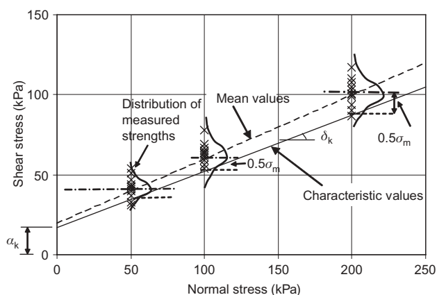
Figure 1. Derivation of interface shear strength parameters from measured shear strengths
