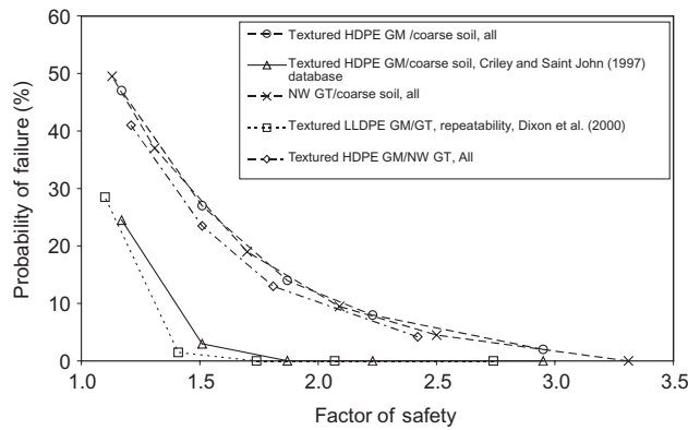
Figure 15. Probability of failure against factor of safety from veneer stability analysis, presenting data from combined data sets, Criley and Saint John (1997) and Dixon et al. (2000)
