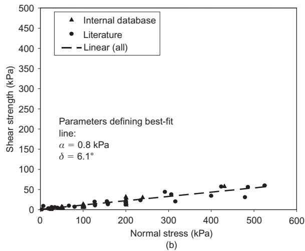
Figure 2. Shear strength against normal stress for smooth HDPE geomembrane/nonwoven geotextile from internal database and literature: (a) peak; (b) large displacement
