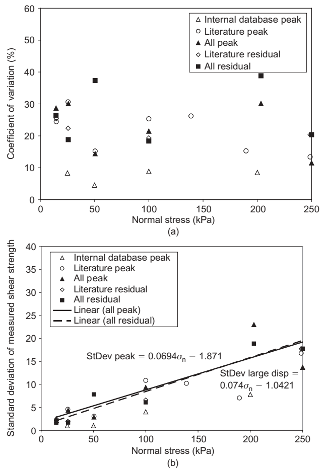
Figure 11. Smooth HDPE geomembrane/coarse soil from internal database, literature and combined for peak and large displacement: (a) coefficient of variation against normal stress; (b) standard deviation of measured shear strength against normal stress
