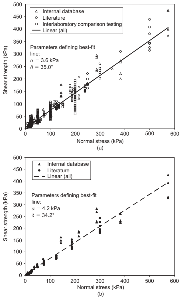
Figure 6. Shear strength against normal stress for nonwoven geotextile/coarse soil from literature, internal database and interlaboratory comparison testing: (a) peak; (b) large displacement
