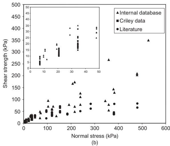
Figure 8. Shear strength against normal stress for textured HDPE geomembrane/fine soil from literature, internal database and Criley and Saint John (1997) repeatability results: (a) peak; (b) large displacement
