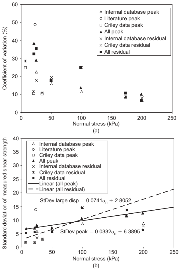
Figure 12. Textured HDPE geomembrane/coarse soil from internal database, literature, Criley and Saint John (1997) repeatability results and combined for peak and large displacement: (a) coefficient of variation against normal stress; (b) standard deviation of measured shear strength against normal stress
