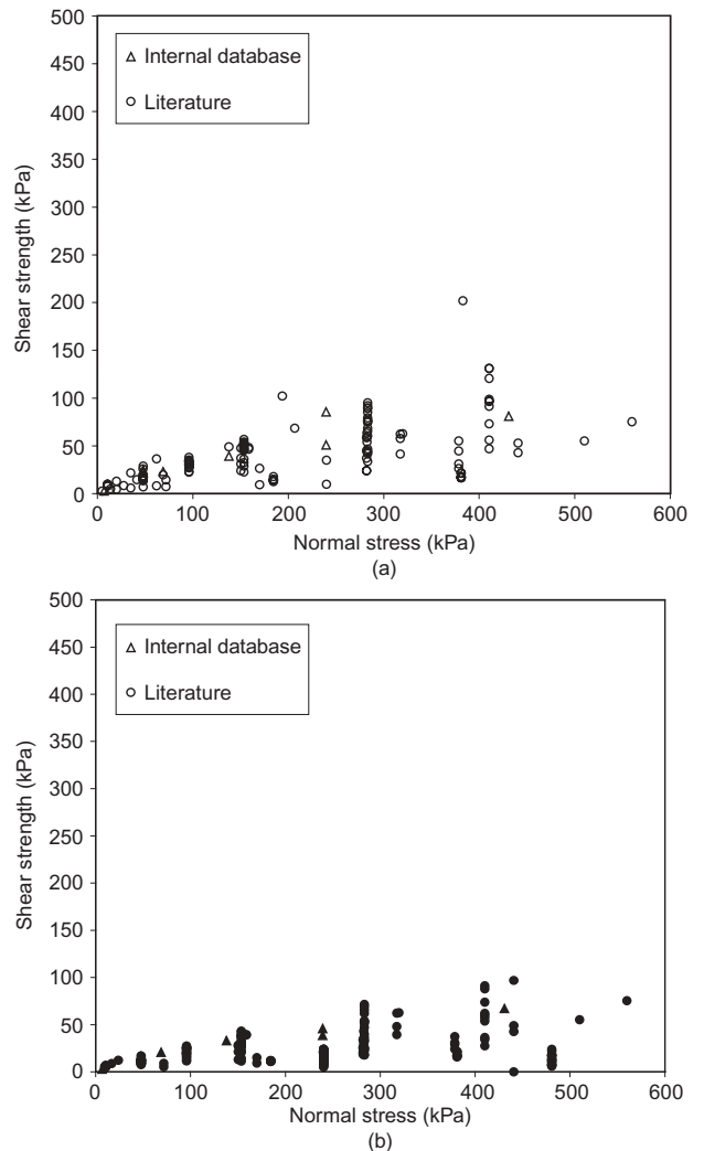
Figure 7. Shear strength against normal stress for smooth HDPE geomembrane/fine soil from literature and internal database: (a) peak; (b) large displacement
