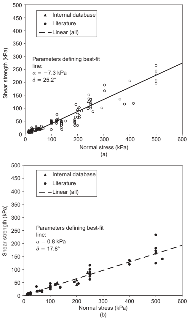
Figure 4. Shear strength against normal stress for smooth HDPE geomembrane/coarse soil from literature and internal database: (a) peak; (b) large displacement
