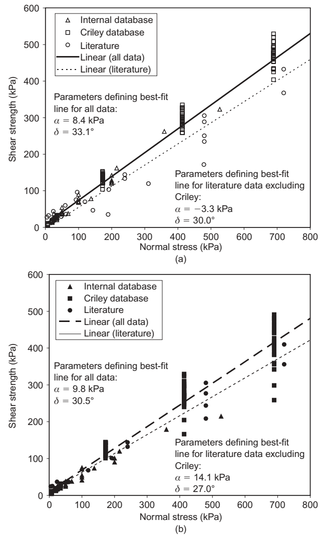
Figure 5. Shear strength against normal stress for textured HDPE geomembrane/coarse soil from literature, internal database, and Criley and Saint John (1997) repeatability results: (a) peak; (b) large displacement
