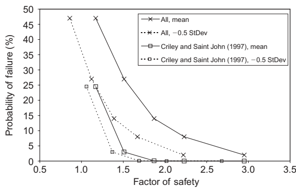
Figure 16. Probability of failure against factor of safety for veneer stability, showing the relationship between the mean and characteristic values for factor of safety, based on combined data and Criley and Saint John (1997) for textured HDPE geomembrane/coarse soil
