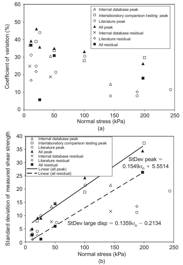
Figure 13. Nonwoven geotextile/coarse soil from literature, internal database, interlaboratory comparison testing and combined for peak and large displacement: (a) coefficient of variation against normal stress; (b) standard deviation of measured shear strength against normal stress
