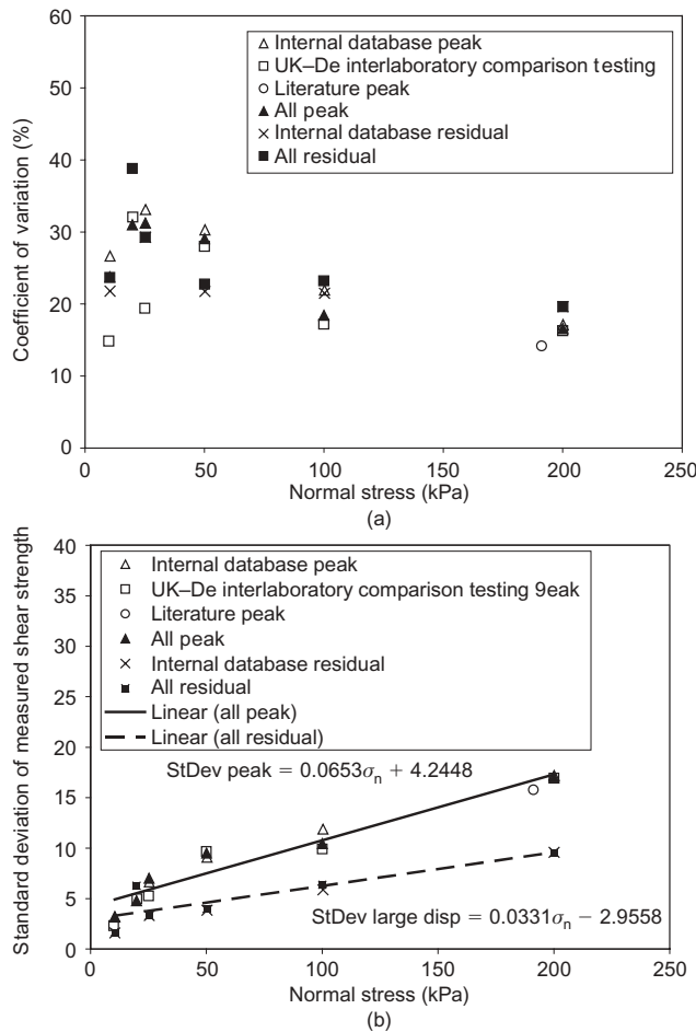
Figure 10. Textured HDPE geomembrane/nonwoven geotextile from internal database, literature, interlaboratory comparison tests and combined for peak and large displacement: (a) coefficient of variation against normal stress; (b) standard deviation of measured shear strength against normal stress
